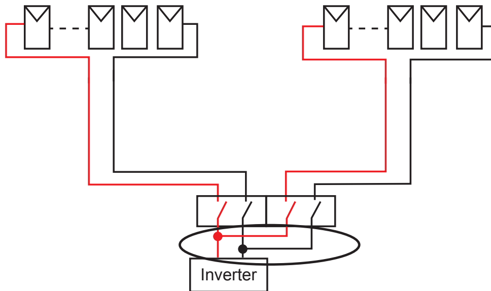
Figure 22: Paralleling strings on inverter/MPPT side of PV array disconnector devices
