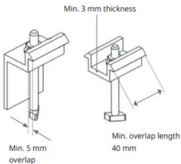
Figure 21: Module Clamps (Source: Canadian Solar)
