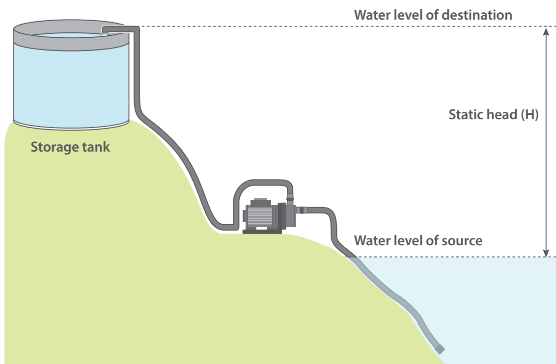
Figure 9: Total static head of a solar water pumping system
