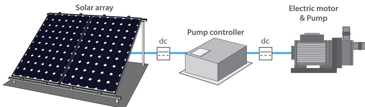
Figure 2: dc powered pump
