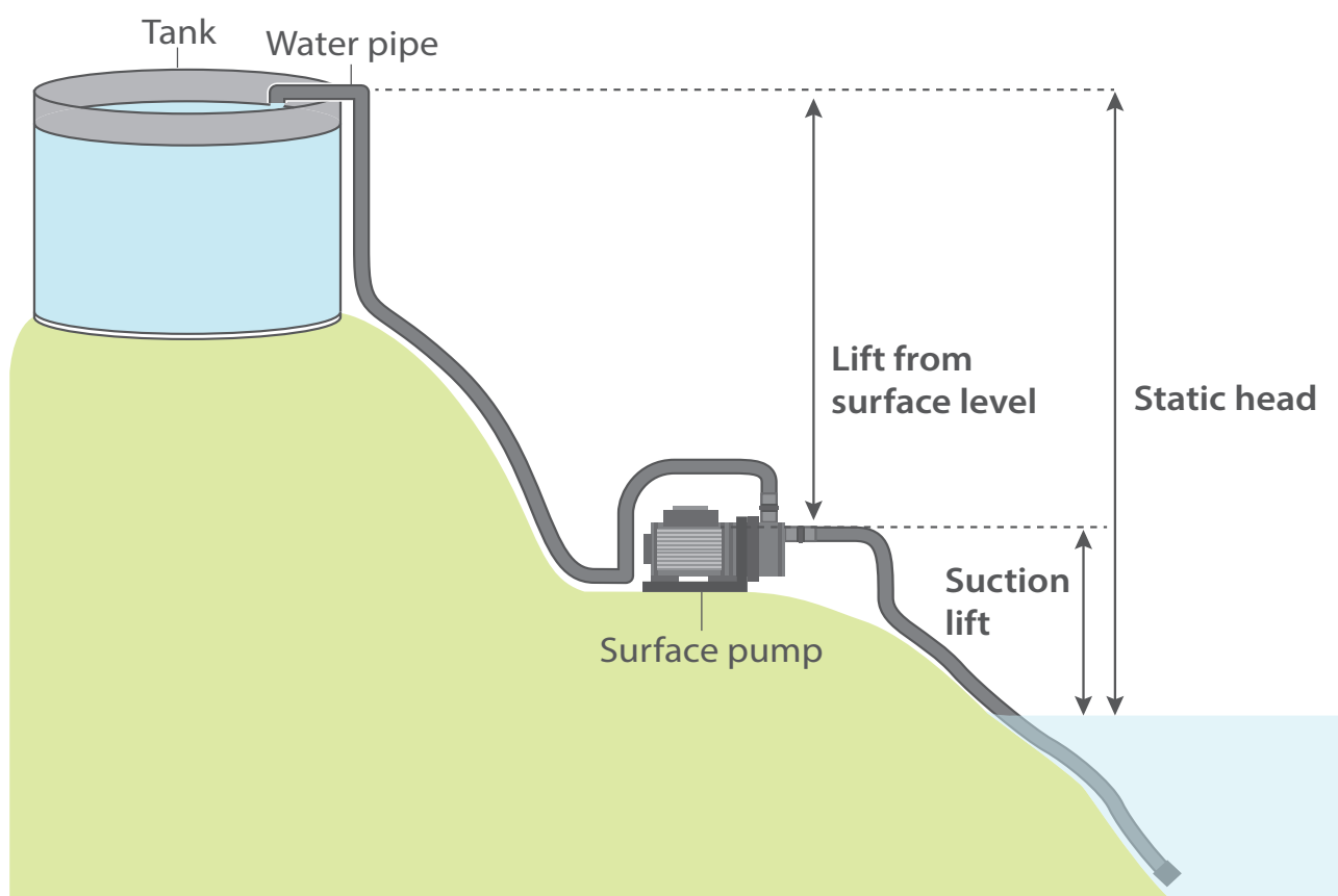
Figure 11: Static Head for Surface Level Pump
